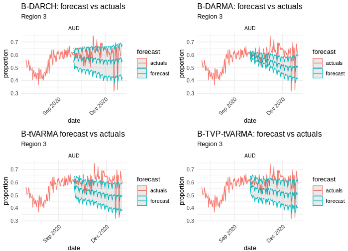
Fig. 5. Airbnb data analysis: Region 3 – 92-day forecasts (blue) with 95% credible intervals (shaded) for the AUD currency from Oct. 1 to Dec. 31, 2020, compared to actual values (red) from the preceding six months. Models shown: B-DARCH, B-DARMA, B-tVARMA, and B-TVP-tVARMA. (For interpretation of the references to colour in this figure legend, the reader is referred to the web version of this article.)
