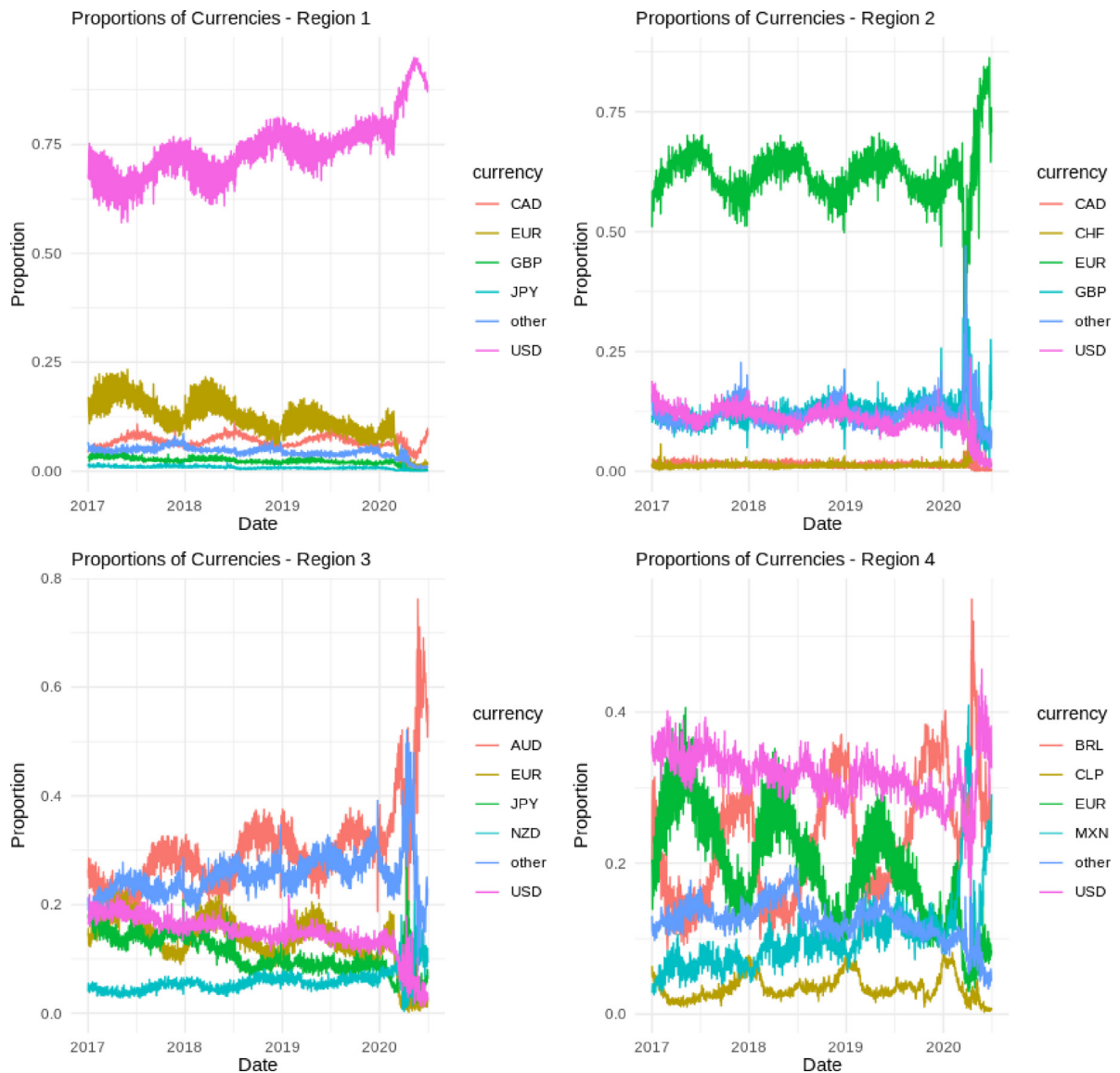
Fig. 1. Airbnb data analysis: Proportion of fees by billing currency for four regions from Jan 1, 2017, to June 30, 2020. AUD is the Australian dollar, BRL is the Brazilian real, CAD is the Canadian dollar, CHF is the Swiss franc, CLP is the Chilean peso, EUR is the European euro, GBP is the British pound, MXN is the Mexican peso, NZD is the New Zealand dollar, and USD is the U.S. dollar.
