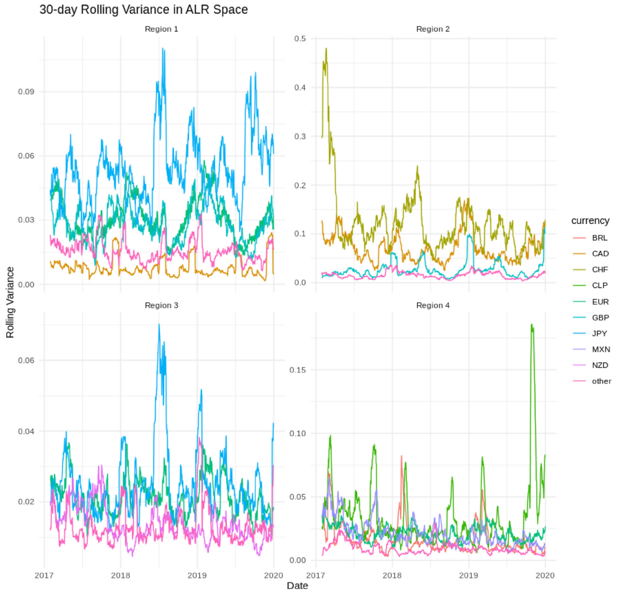
Fig. 2. Airbnb data analysis: Proportion of fees by currency – 30-day rolling ALR variance for four regions from Jan 1, 2017, to Dec 31, 2019. USD is the reference component.
