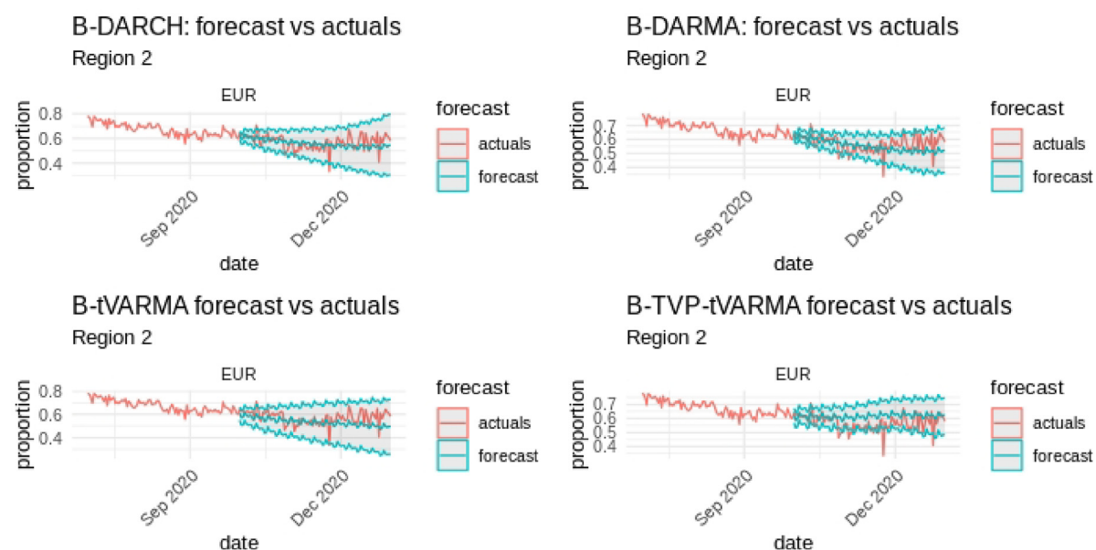
Fig. 4. Airbnb data analysis: Region 2 – 92-day forecasts (blue) with 95% credible intervals (shaded) for the EUR currency from Oct. 1 to Dec. 31, 2020, compared to actual values (red) from the preceding six months. Models shown: B-DARCH, B-DARMA, B-tVARMA, and B-TVP-tVARMA. (For interpretation of the references to colour in this figure legend, the reader is referred to the web version of this article.)
