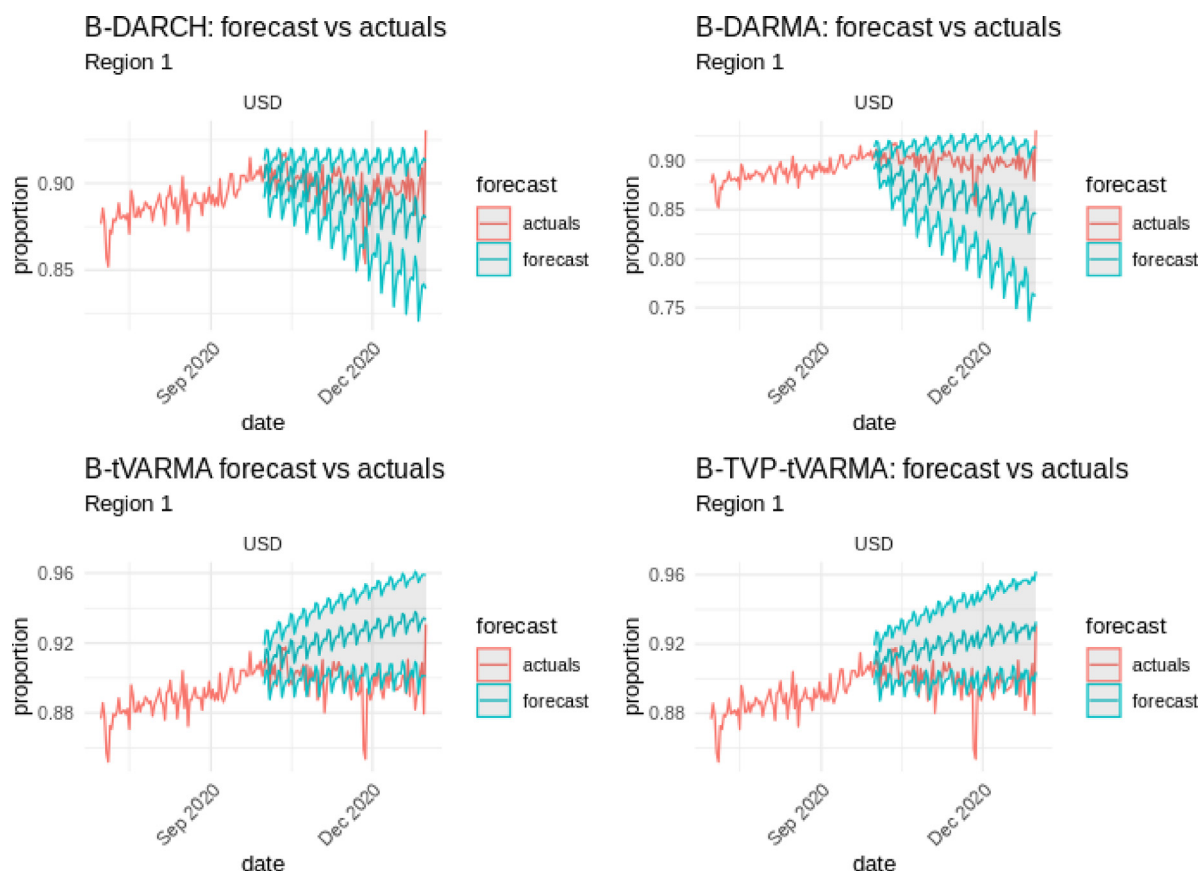
Fig. 3. Airbnb data analysis: Region 1 – 92-day forecasts (blue) with 95% credible intervals (shaded) for the USD currency from Oct. 1 to Dec. 31, 2020, compared to actual values (red) from the preceding six months. Models shown: B-DARCH, B-DARMA, B-tVARMA, and B-TVP-tVARMA. (For interpretation of the references to colour in this figure legend, the reader is referred to the web version of this article.)
