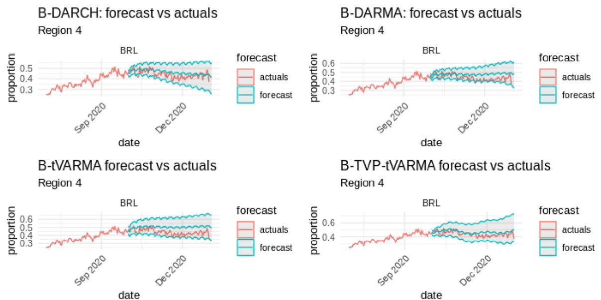
Fig. 6. Airbnb data analysis: Region 4 – 92-day forecasts (blue) with 95% credible intervals (shaded) for the BRL currency from Oct. 1 to Dec. 31, 2020, compared to actual values (red) from the preceding six months. Models shown: B-DARCH, B-DARMA, B-tVARMA, and B-TVP-tVARMA. (For interpretation of the references to colour in this figure legend, the reader is referred to the web version of this article.)
